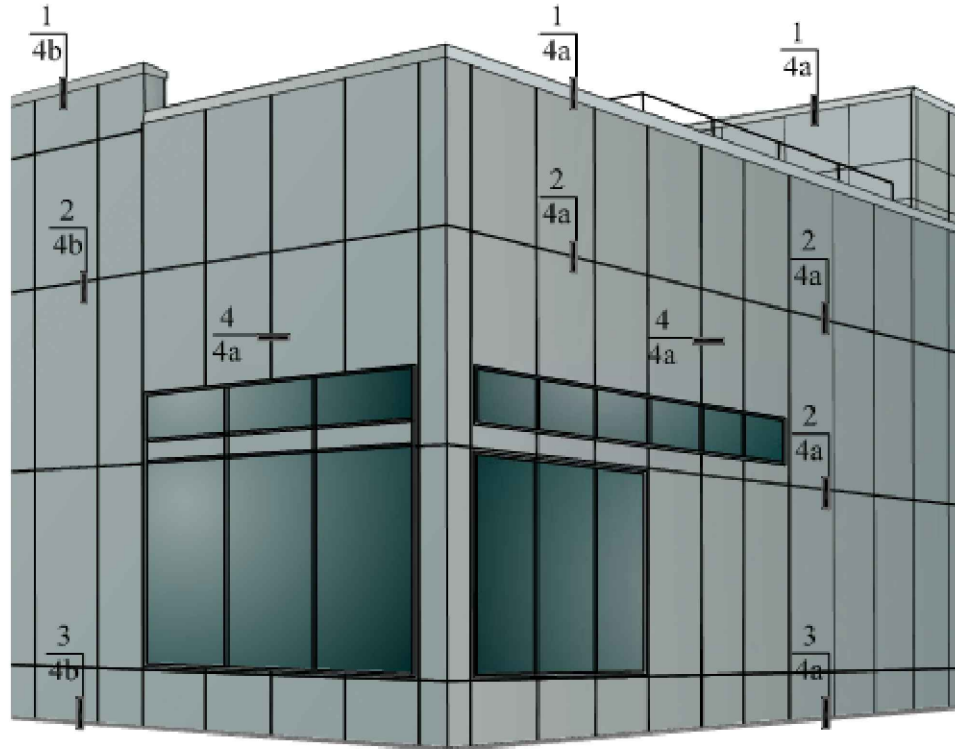
PARTIAL ELEVATION
